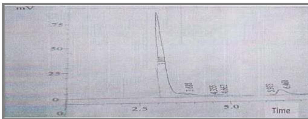
Figure 1. Stander of Gallic acid analyzed by HPLC . Retention Time of Gallic acid (RT) is 3.00
