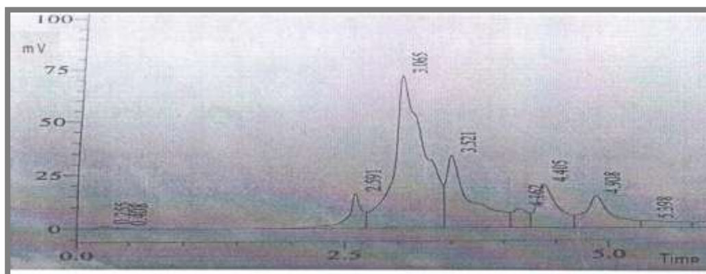
Figure 2. Gallic acid of Scenedesmus sp. analyzed by HPLC . Retention Time of Gallic acid (RT) is 3.06
