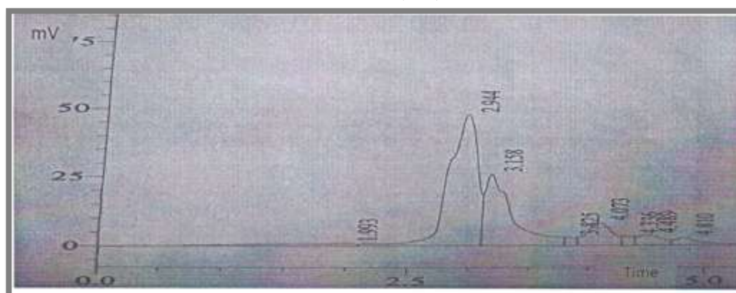
Figure 3. Gallic acid of Oscillatoria sp. analyzed by HPLC . Retention Time of Gallic acid (RT) is ( 2.94 )
